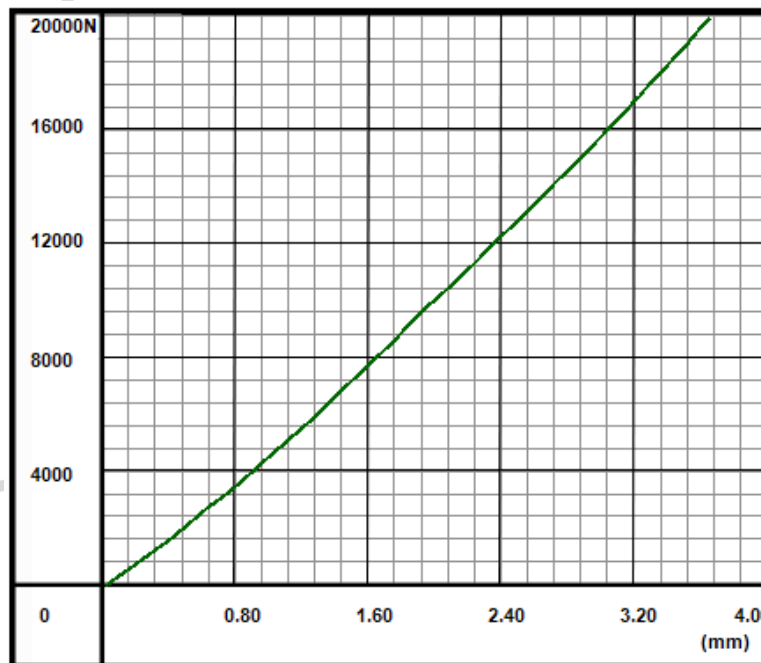
Compression Curve
